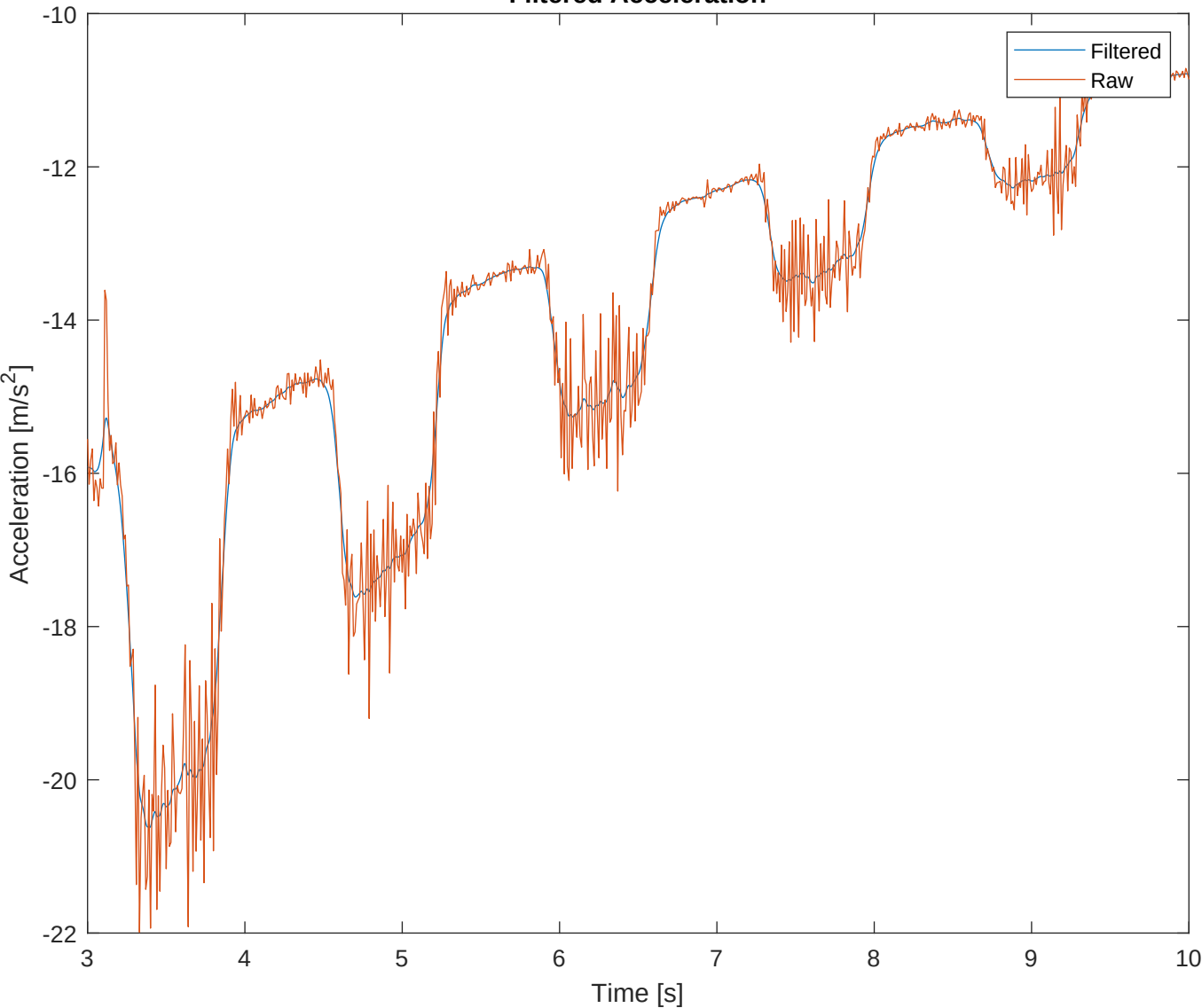
Filtered Acceleration
